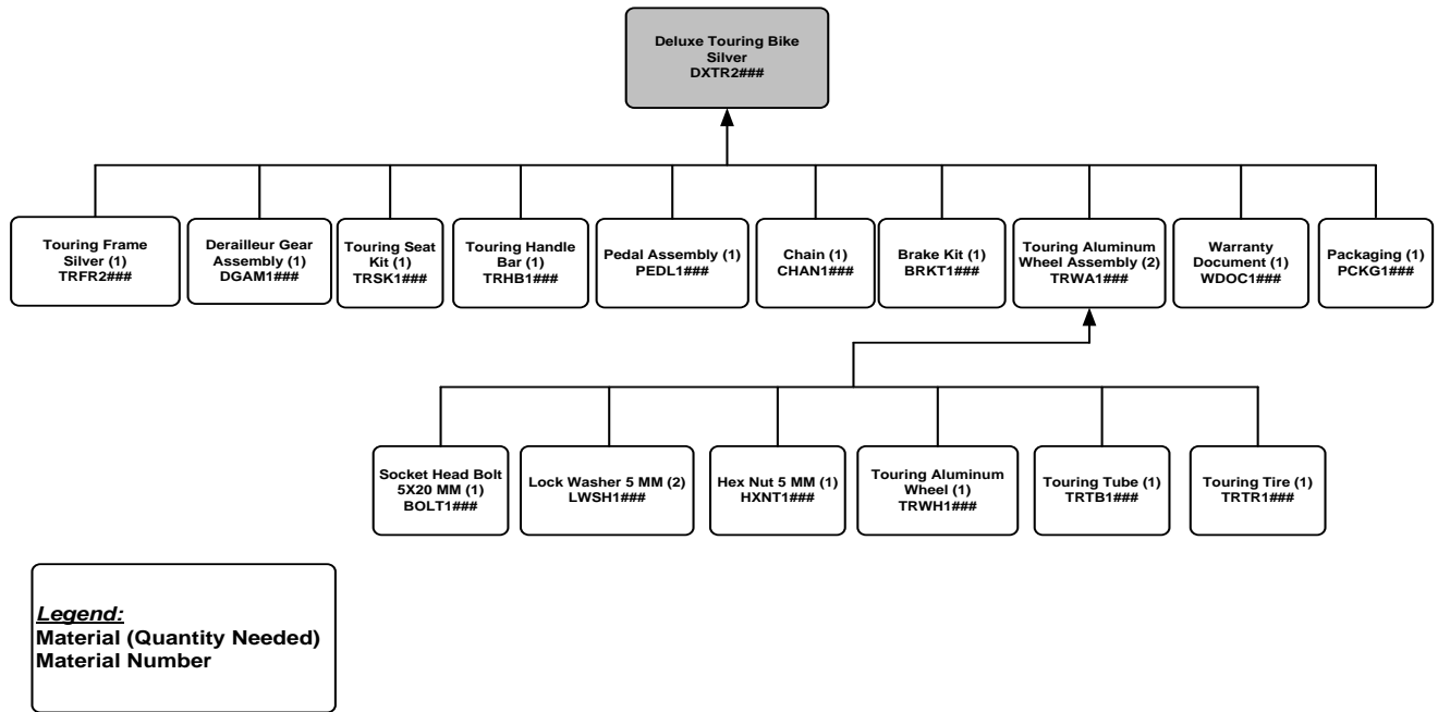
Figure 1: Deluxe Touring Bike (Silver) Bill of Materials
